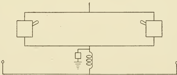
Fig. 128. Parallel Connections of Circuit Breakers Requiring but One Lightning Arrester
